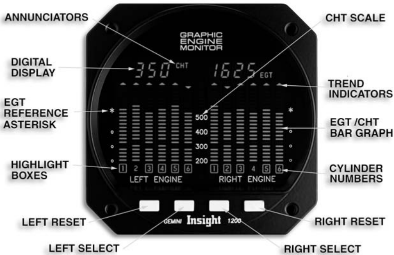
Figure 7. GEMINI 1200 Display
