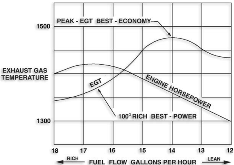
Figure 1 EGT/Fuel Flow Curve
