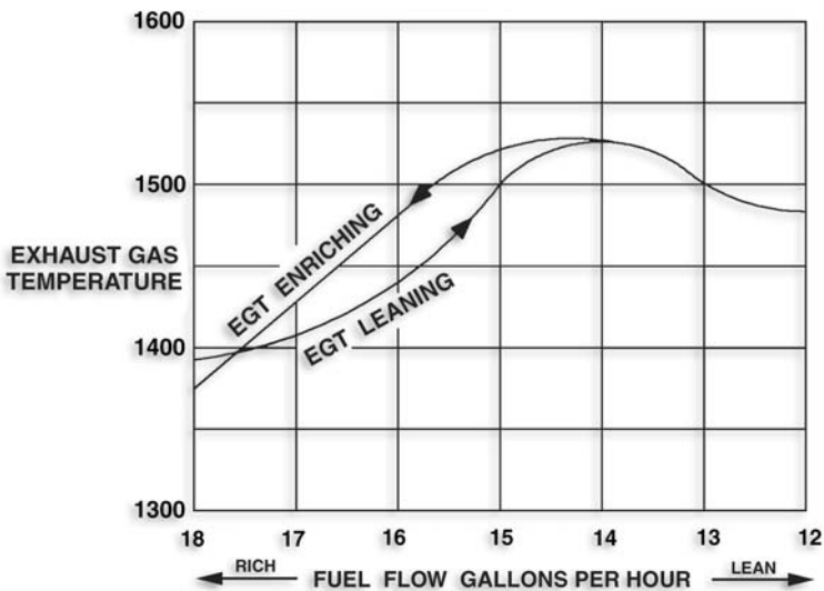
Figure 4. EGT/Fuel Flow for Turbos
