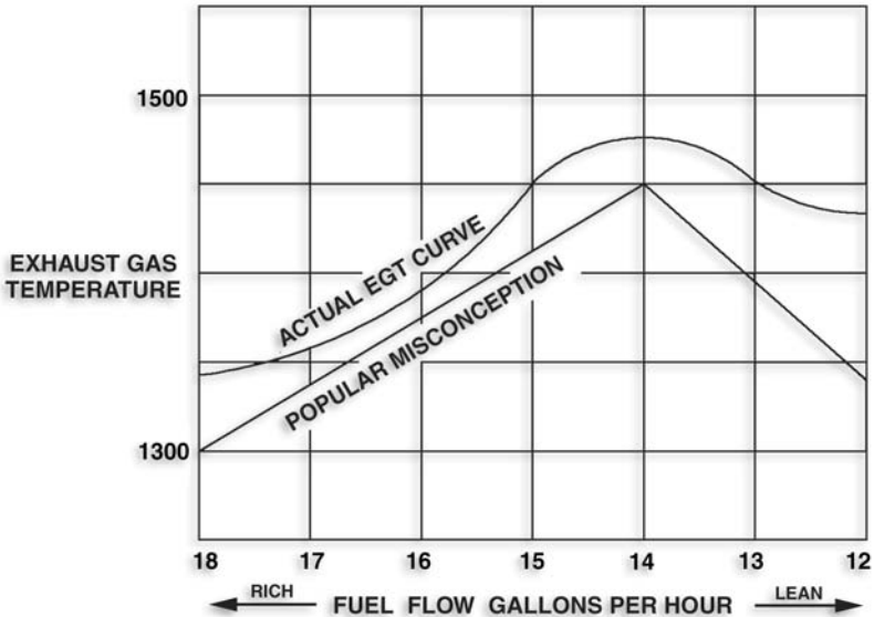
Figure 2 EGT Curves: Fact and Fiction
